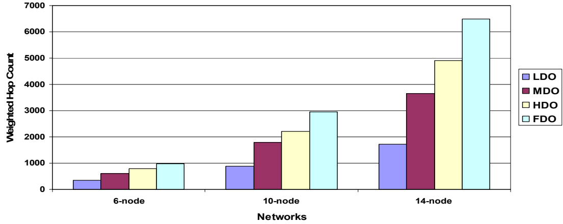
Figure 3.3: Resource requirements vs. network size with |K| = 16 in fault-free networks with wavelength conversion.
